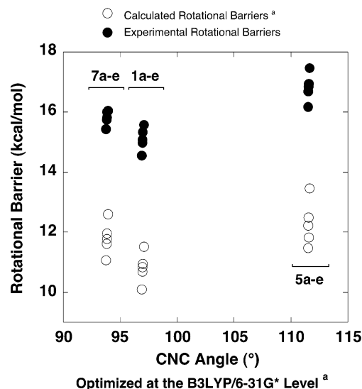
Figure 9. Relationship between calculated CNC angles and experimental or calculated rotational barriers. Calculations were performed at the B3LYP/6-311G**//B3LYP/6-31G* level.
