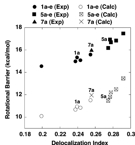
Figure 11. Relationship between electron delocalization from n_N to \pi^*_{CO} calculated by the bond model and the experimental/calculated rotational barriers.
